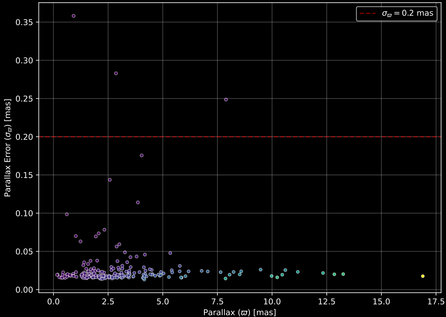
APOGEE DR17 Field: [107-46_MGA] Parallax Quality (n= 200)
