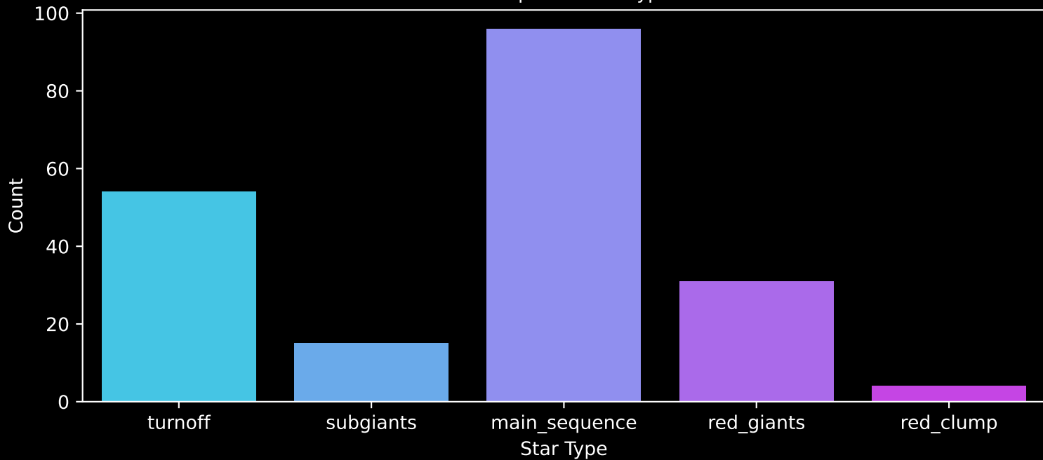
APOGEE DR17 Field: [107-46_MGA] Count plot of Star Type
