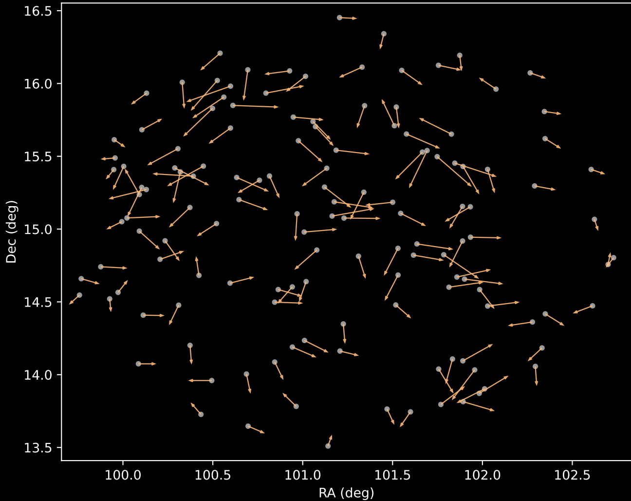
APOGEE DR17 Cluster 3 Proper Motion Vectors (n=136)
