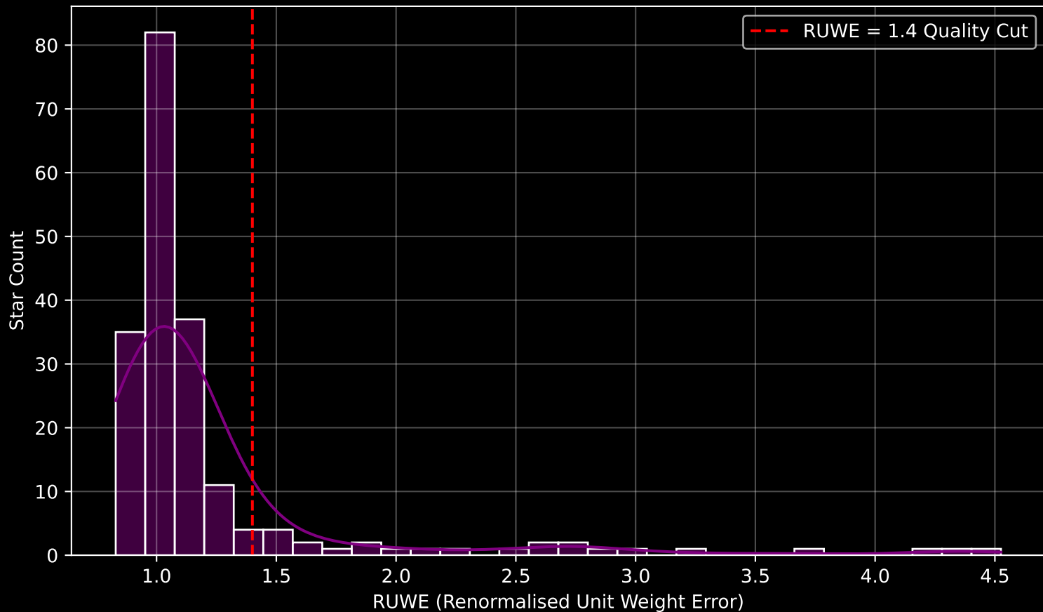
GAPOGEE DR17 Field [107-46_MGA] RUWE Distribution (n= 193)
