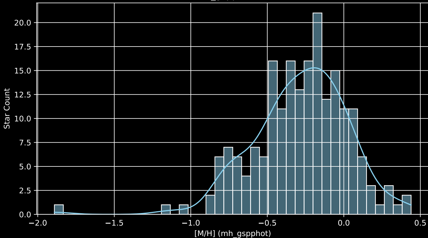
APOGEE DR17 Field: [107-46_MGA [M/H] (mh_gspphot) (n= 199)
