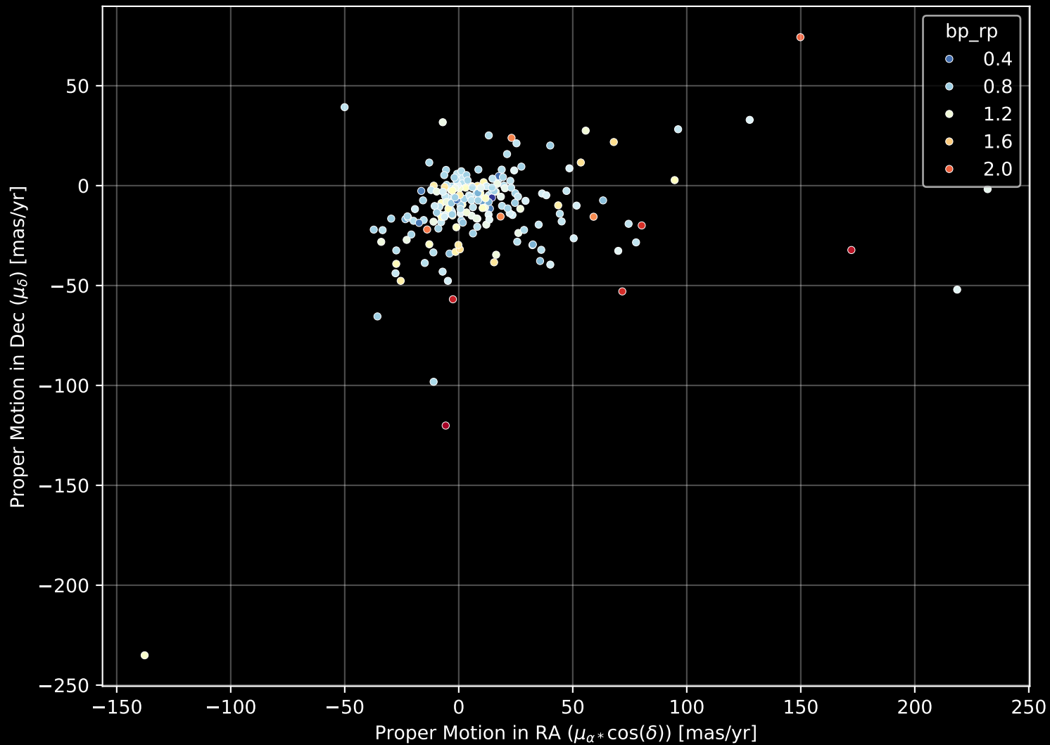
APOGEE DR17 Field: [107-46_MGA] Proper Motion Diagram (n= 200)
