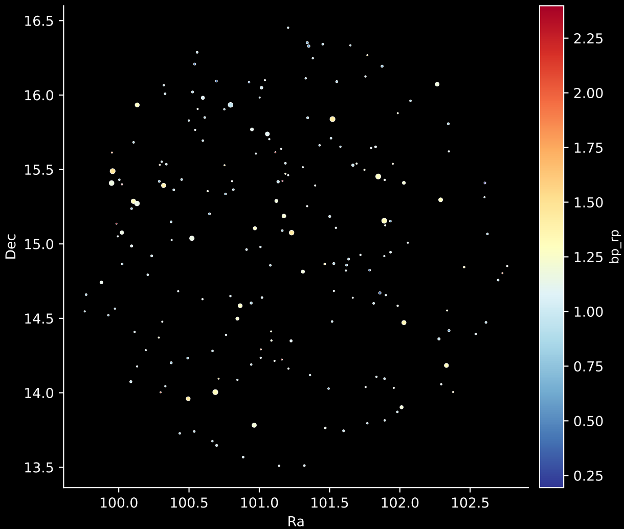
APOGEE DR17 Field: [107-46_MGA] Stars: 200
